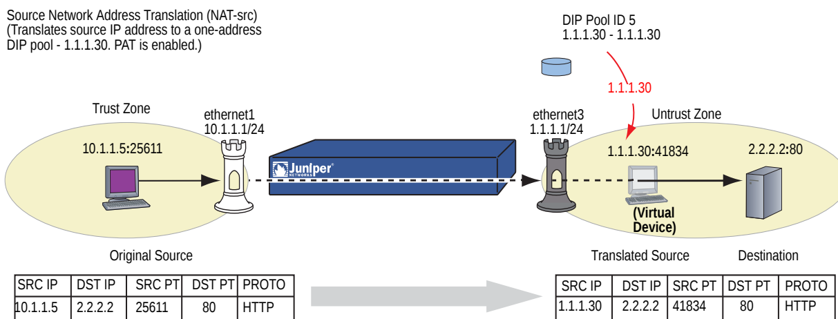
Figure 18: NAT-Src with PAT Enabled
