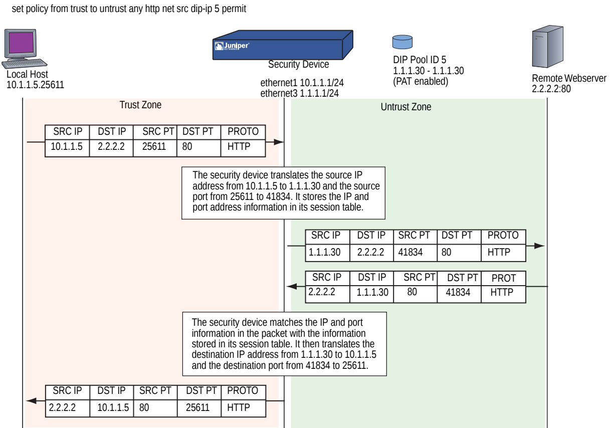
Figure 17: NAT-Src Using a DIP Pool with PAT Enabled
