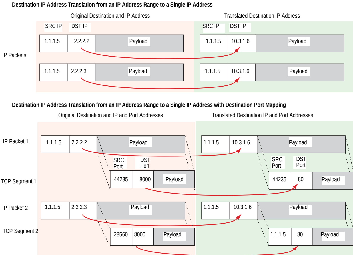
Figure 5: NAT-Dst from an IP Address Range to a Single IP Address
