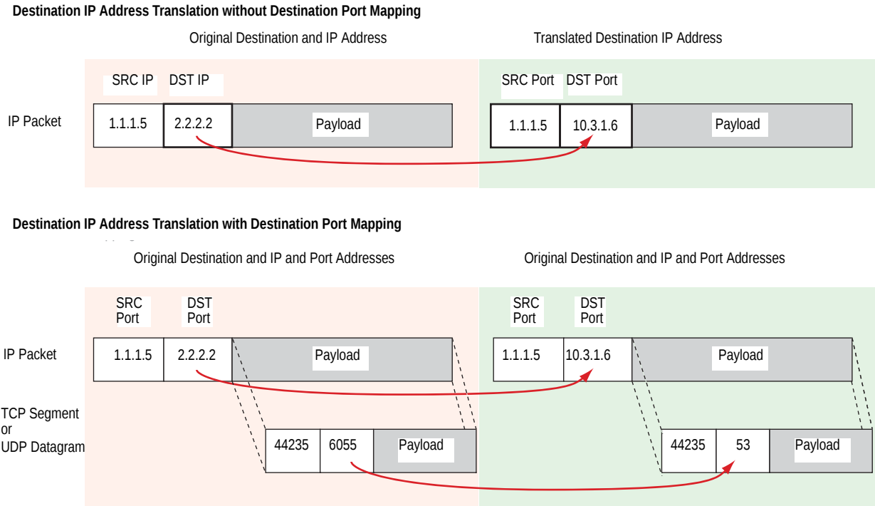
Figure 4: Destination IP Address Translation
