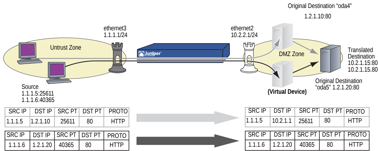
Figure 30: NAT-Dst—Many-to-One
