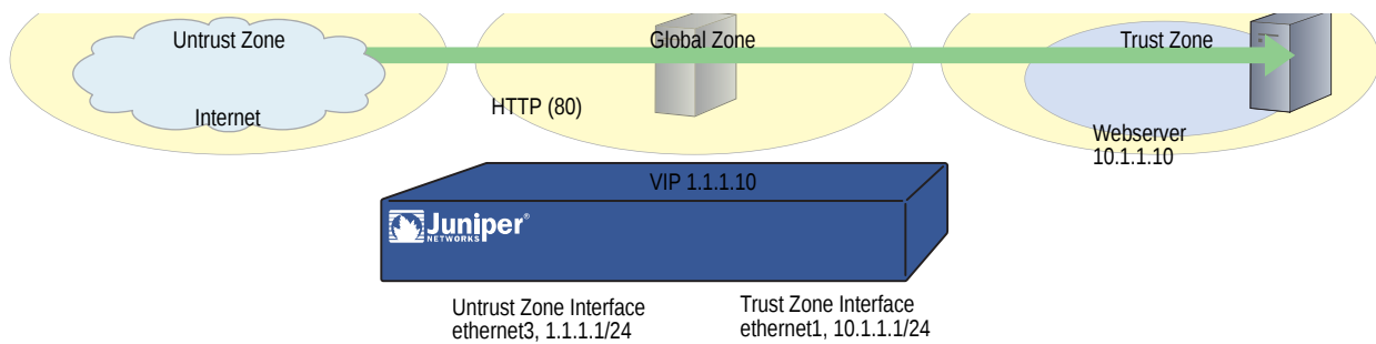
Figure 39: Virtual IP Server
