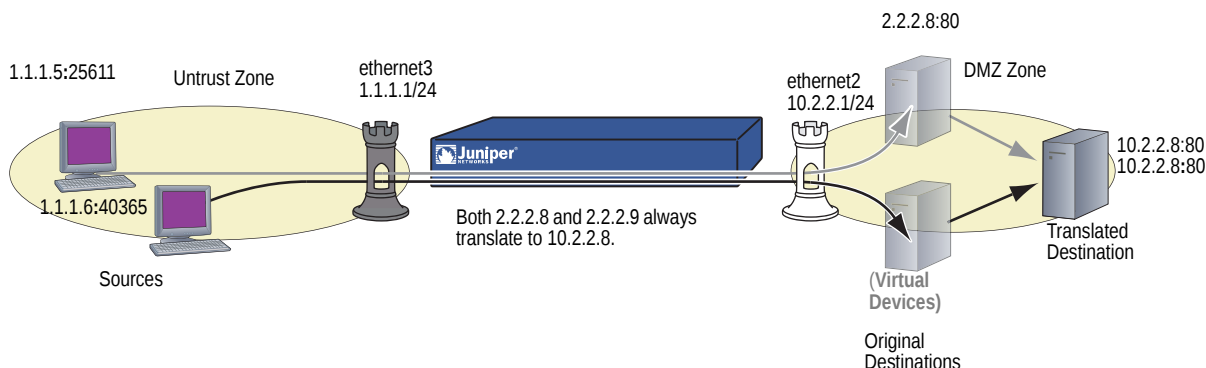
Figure 13: NAT-Dst from an Address Range to a Single IP Address
