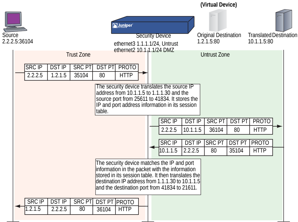
Figure 27: One-to-One NAT-Dst
