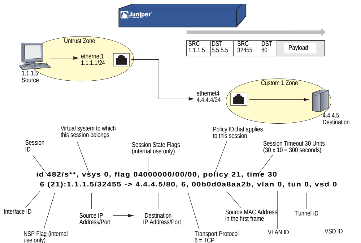
Figure 23: NAT-Dst Packet Flow—Packet Forwarding
